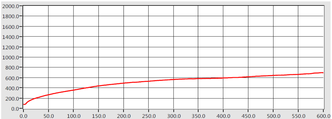
Graph No. 3 - Tunnel Air Temperature (F) Versus Time (sec)
